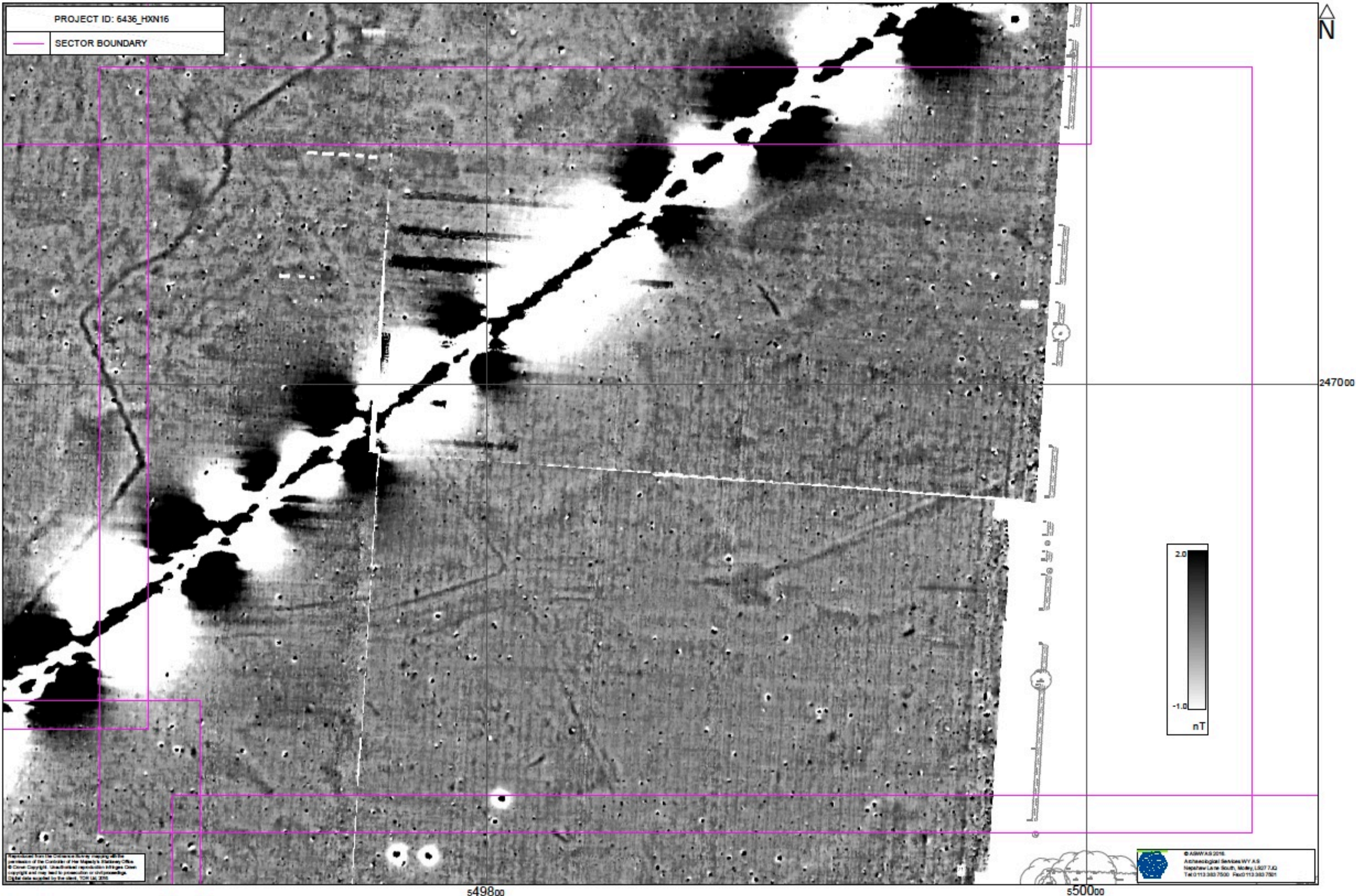
Fig. 16. Processed greyscale magnetometer data; Sector 7 (1:1000 @ A3)
