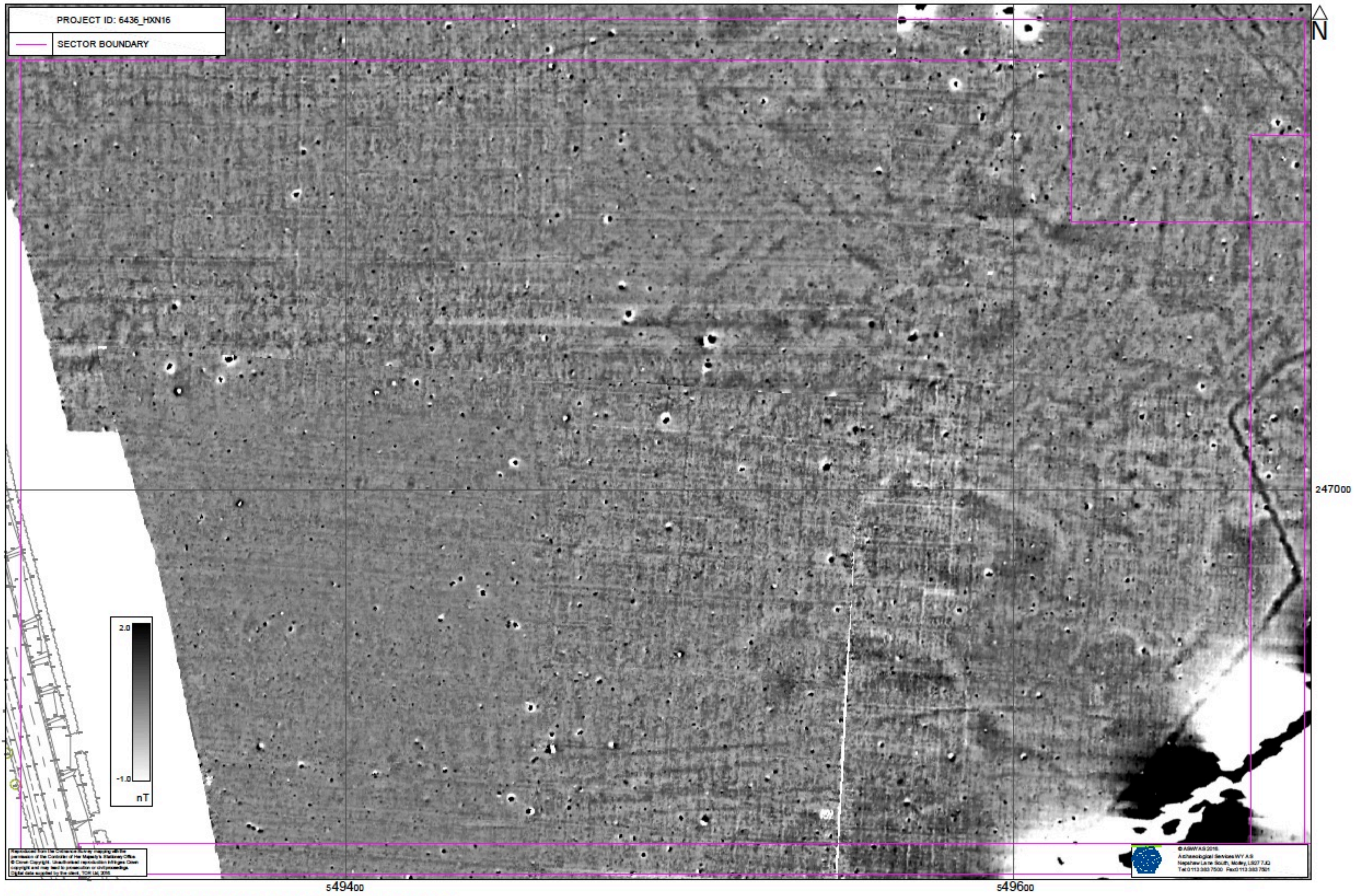
Fig. 14. Processed greyscale magnetometer data; Sector 6 (1:1000 @ A3)
